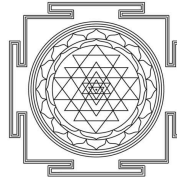
Shri Yantra
